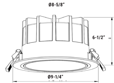
50W DIMENSIONS:
